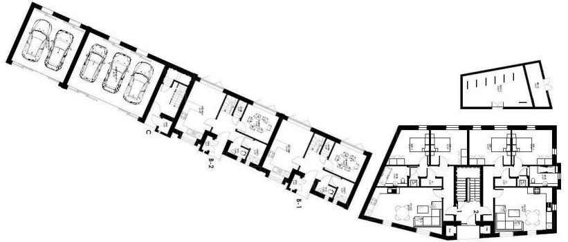
PROPOSED GROUND FLOOR PLANS
